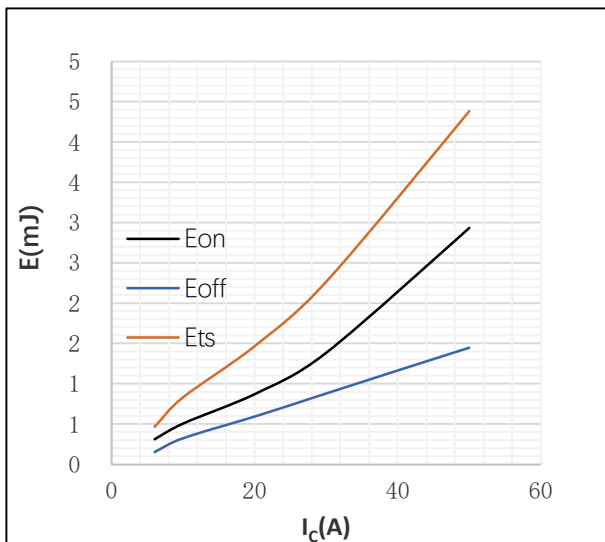
● Fig.15 Switching energy losses as a function of collector current; typical values
