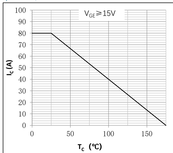
● Fig.6 Continuous collector current as a function of case temperature 2 ; Calculative values
